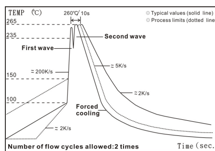
Wave Soldering (Flow Soldering)
